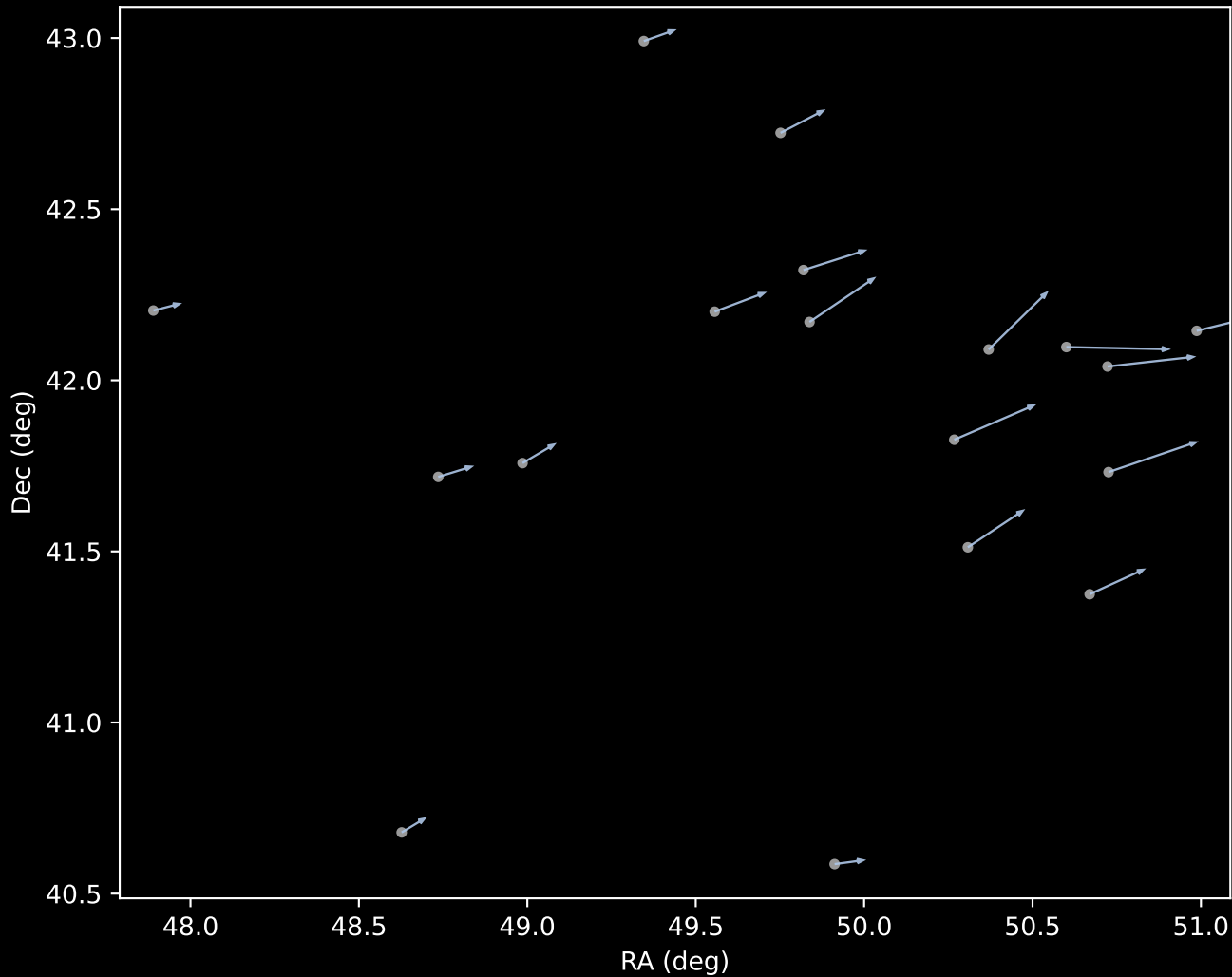
APOGEE DR17 Cluster 1 Proper Motion Vectors (n=18)
