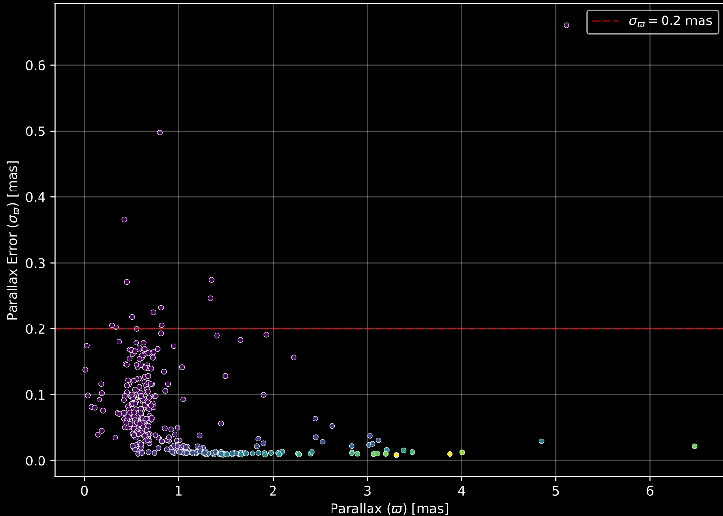
APOGEE DR17 Field: [CygnusX_N_btx] Parallax Quality (n= 349)
