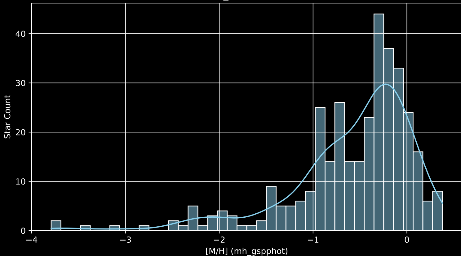
APOGEE DR17 Field: [CygnusX_N_btx [M/H] (mh_gspphot) (n= 345)
