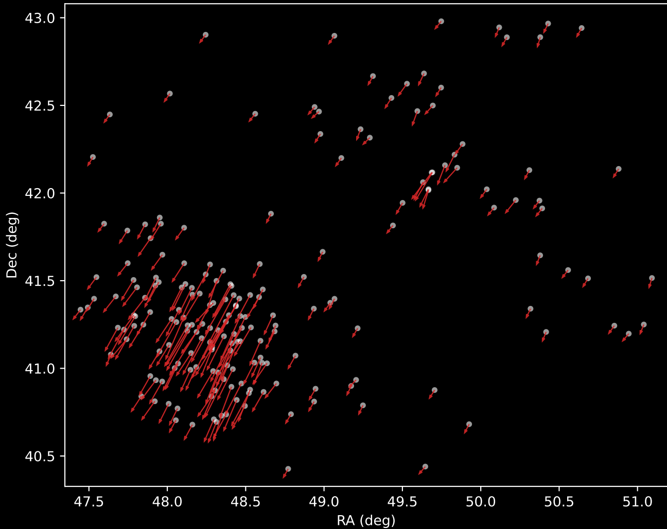
APOGEE DR17 Cluster 6 Proper Motion Vectors (n=192)
