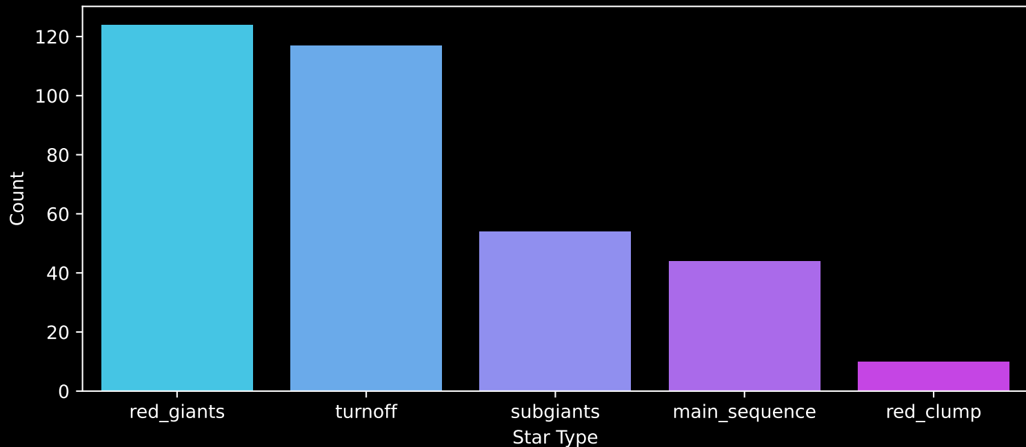
APOGEE DR17 Field: [CygnusX_N_btx] Count plot of Star Type
