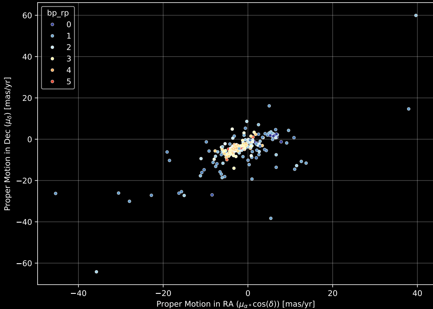
APOGEE DR17 Field: [CygnusX_N_btx] Proper Motion Diagram (n= 349)
