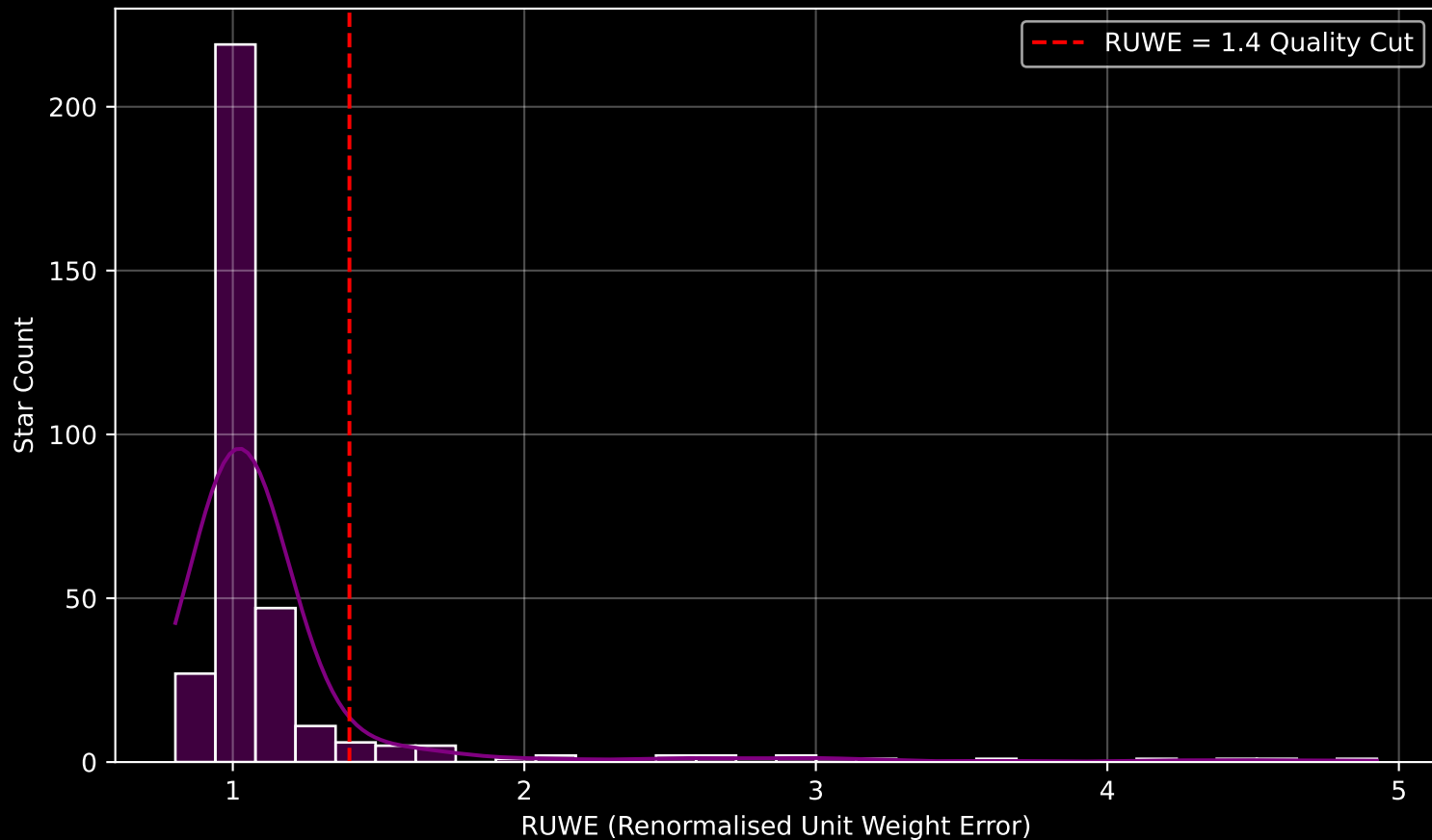
GAPOGEE DR17 Field [CygnusX_N_btx] RUWE Distribution (n= 336)
